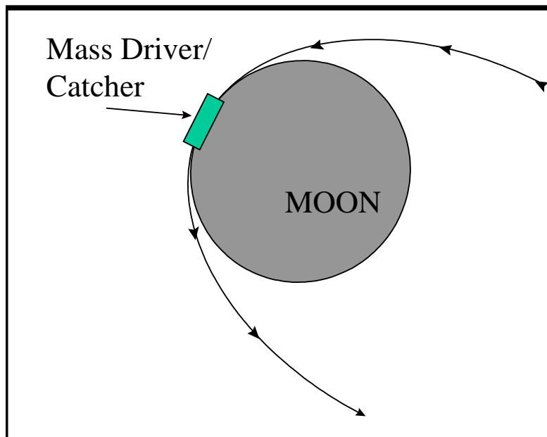
Figure 4: Mass driver on the Moon. Electromagnetic mass drivers will launch and recover spacecraft to and from cis-lunar space, thus eliminating the need for rockets on the Moon. 11
